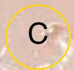
Vitamin C
